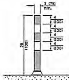
FLEXIBLE DELINEATOR
