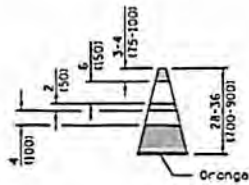
REFLECTORIZED CONE
