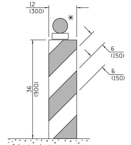
VERTICAL BARRICADE
