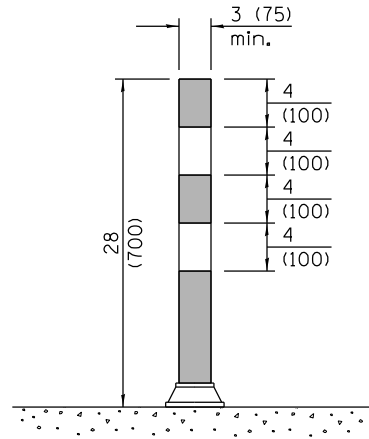
FLEXIBLE DELINEATOR
